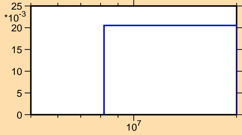
\sigma vs. E for ^{119}\text{In}(n,3n)
