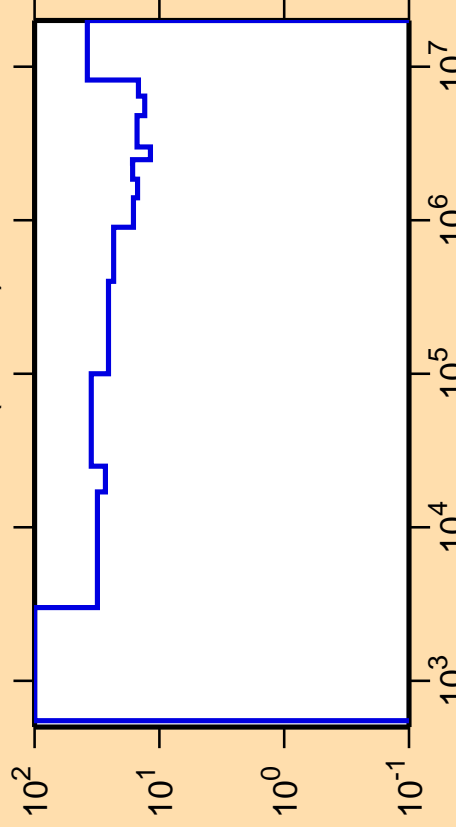
\Delta\sigma/\sigma vs. E for ^{119}\text{In}(n,\text{inel.})
