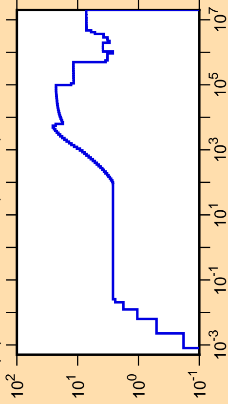
\Delta\mu/\mu vs. E for ^{120}\text{In}(\text{mt251})
