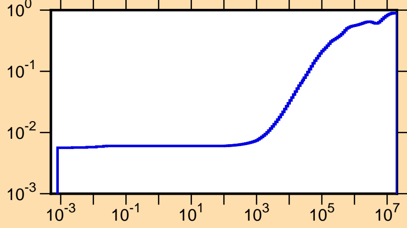
\mu vs. E for ^{120}\text{In}(\text{mt251})
