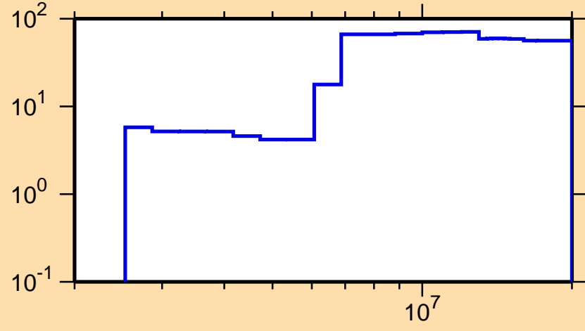
\Delta\sigma/\sigma vs. E for ^{120}\text{In}(n,ncont.)
