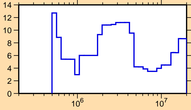
\Delta\sigma/\sigma vs. E for ^{120}\text{In}(n, el.)
