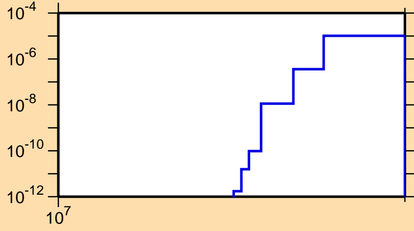
\sigma vs. E for ^{120}\text{In}(n,nd)
