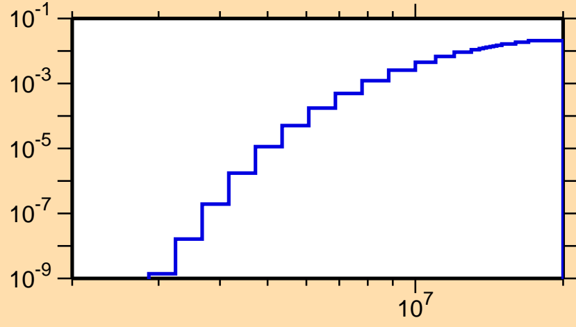
\sigma vs. E for ^{120}\text{In}(n,p)
