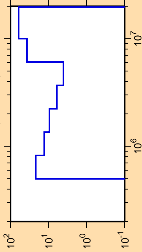
\Delta\sigma/\sigma vs. E for ^{120}\text{In}(n,\text{ncont.})
