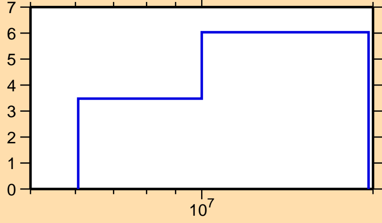
\Delta\sigma/\sigma vs. E for ^{120}\text{In}(n,\text{el.})
