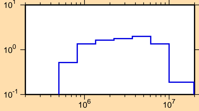
\sigma vs. E for ^{120}\text{In}(n,n\text{cont.})
