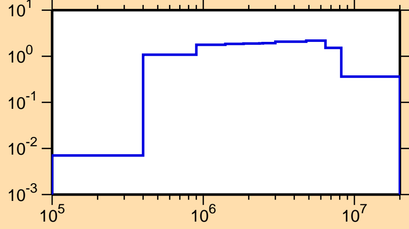
\sigma vs. E for ^{120}\text{In}(n,\text{inel.})
