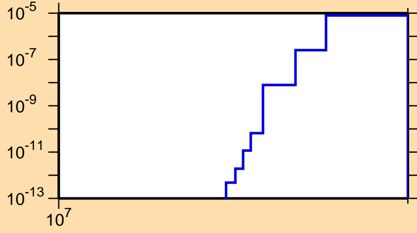
\sigma vs. E for ^{120}\text{In}(n,\text{nd})
