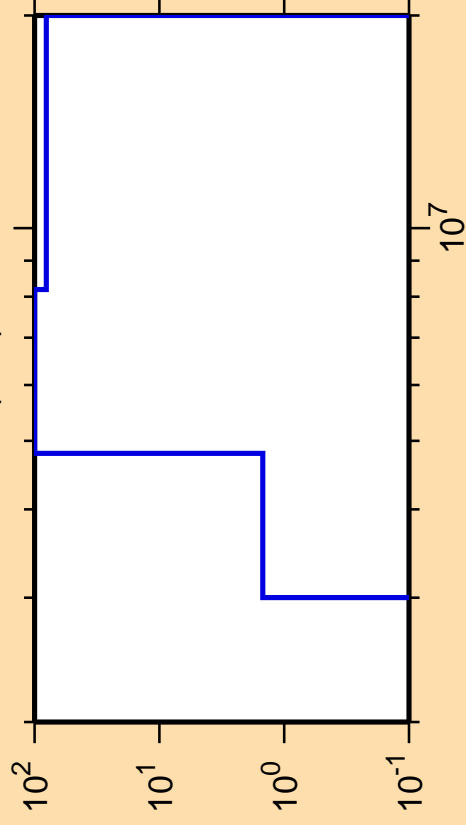
\Delta\sigma/\sigma vs. E for ^{120}\text{In}(n,\alpha)
