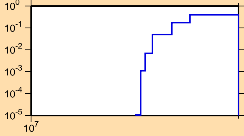
\sigma vs. E for ^{120}\text{In}(n,3n)
