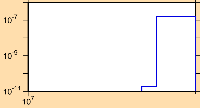
\sigma vs. E for ^{120}\text{In}(n,nt)
