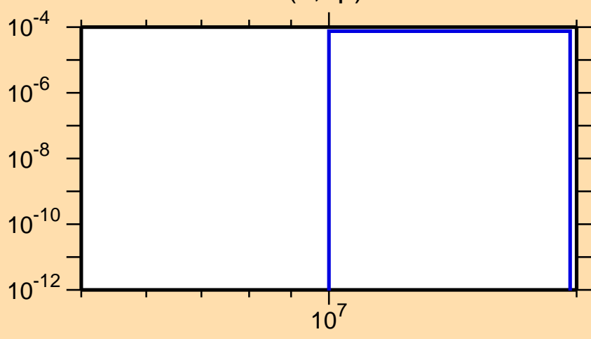
\sigma vs. E for ^{121}\text{In}(n,np)
