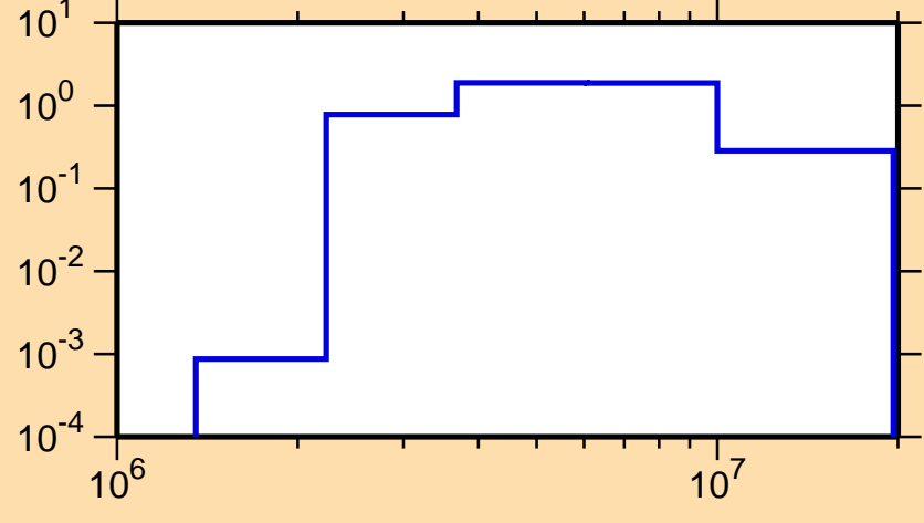
\sigma vs. E for ^{121}\text{In}(n,n\text{cont.})
