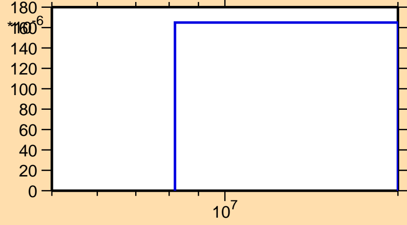
\sigma vs. E for ^{121}\text{In}(n,d)
