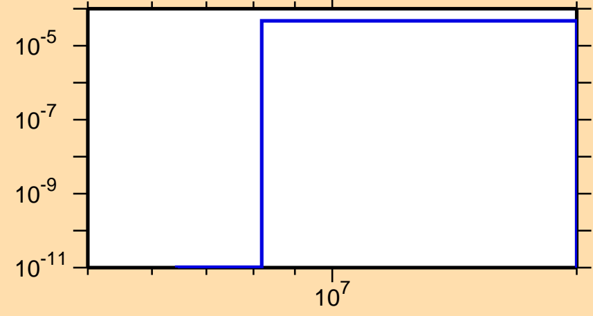
\sigma vs. E for ^{121}\text{In}(n,\alpha)
