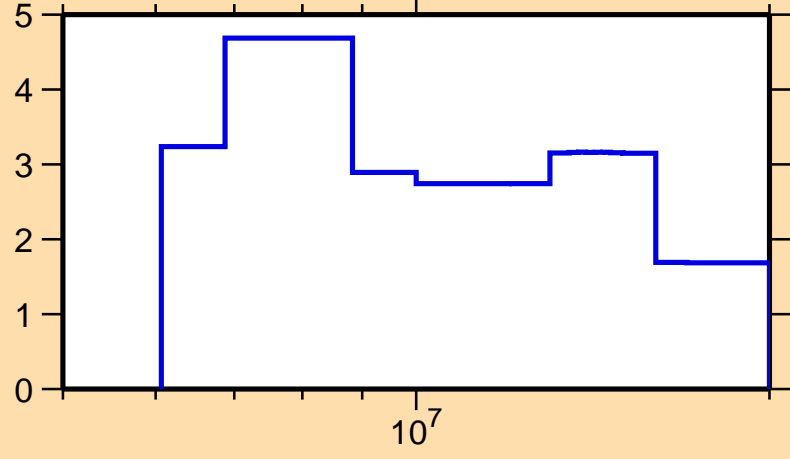
\Delta\sigma/\sigma vs. E for ^{121}\text{In}(n,\text{nonel.})
