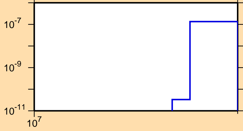
\sigma vs. E for ^{121}\text{In}(n,nt)
