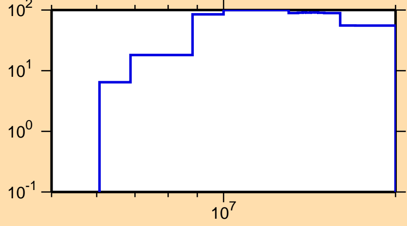
\Delta\sigma/\sigma vs. E for ^{121}\text{In}(n,n\text{cont.})
