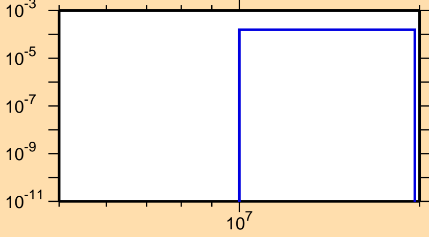
\sigma vs. E for ^{121}\text{In}(n,np)
