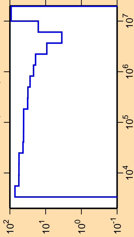
\Delta\sigma/\sigma vs. E for ^{121}\text{In}(n,\text{inel.})
