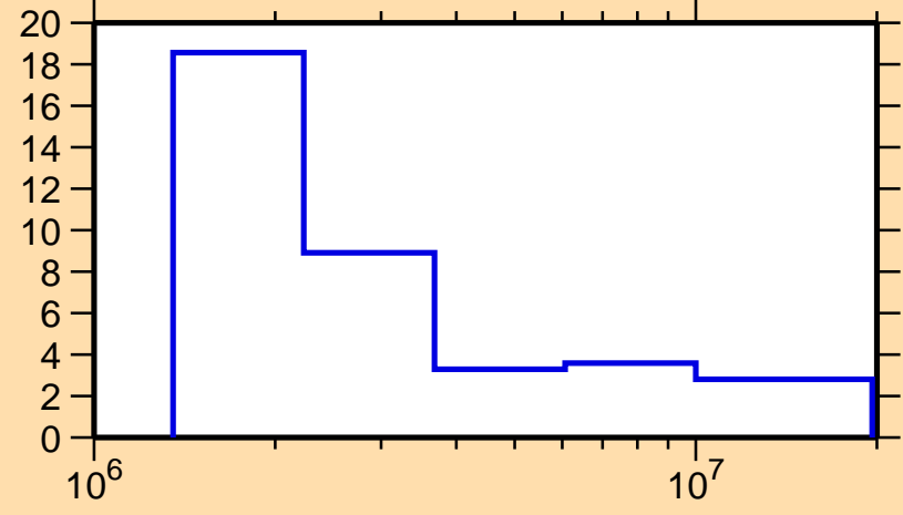
\Delta\sigma/\sigma vs. E for ^{121}\text{In}(n,n\text{nonel.})
