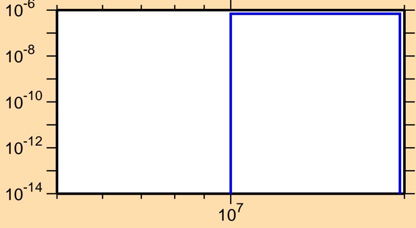
\sigma vs. E for ^{121}\text{In}(n,n\alpha)
