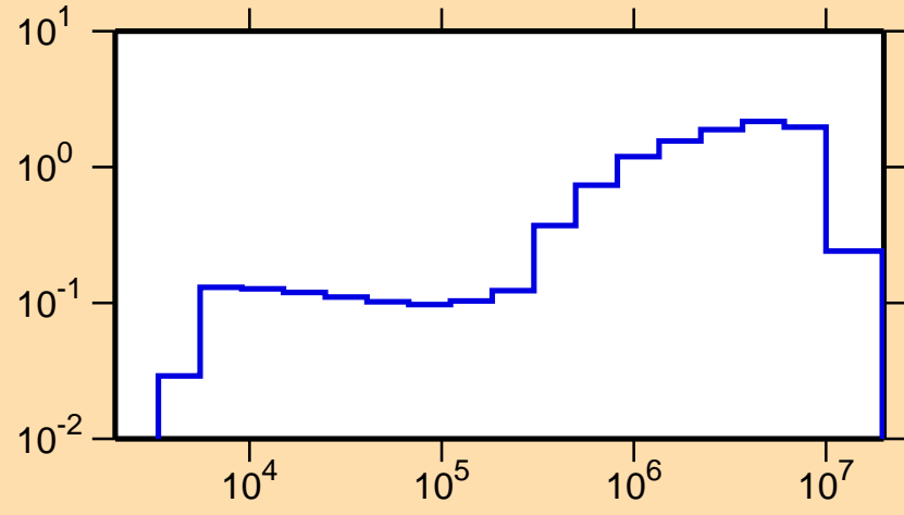
\sigma vs. E for ^{121}\text{In}(n,\text{inel.})
