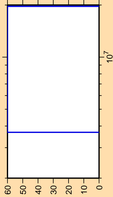
\Delta\sigma/\sigma vs. E for ^{121}\text{In}(n,p)
