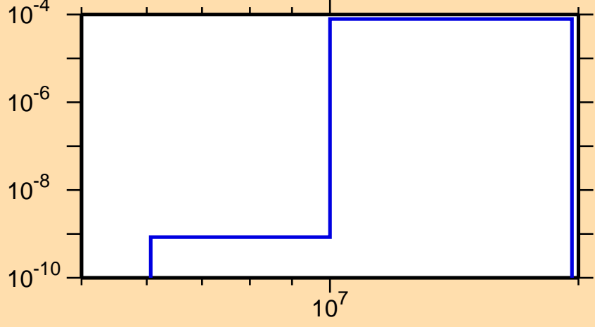
\sigma vs. E for ^{121}\text{In}(n,\alpha)
