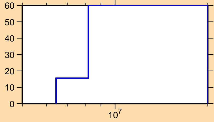
\Delta\sigma/\sigma vs. E for ^{121}\text{In}(n,ncont.)
