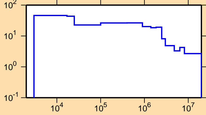
\Delta\sigma/\sigma vs. E for ^{121}\text{In}(n,\text{nonel.})
