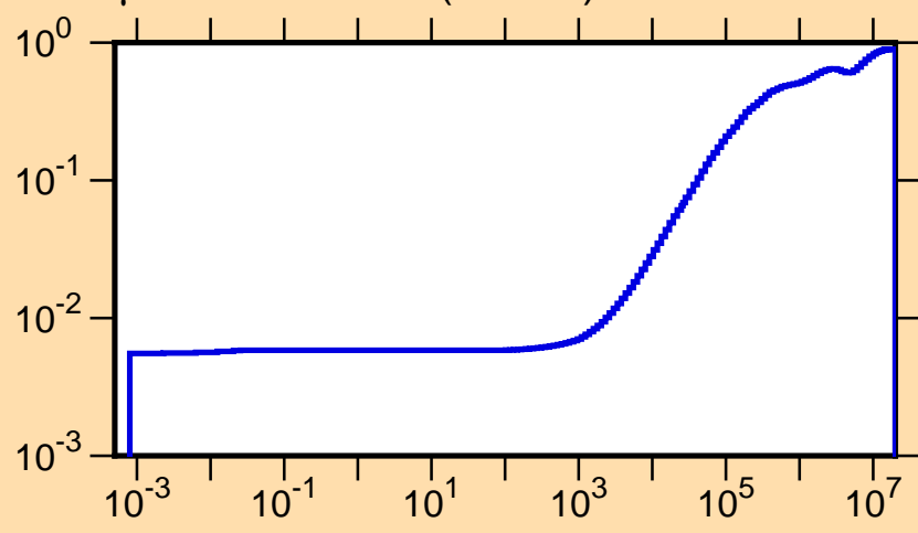
\mu vs. E for ^{122}\text{In}(\text{mt251})
