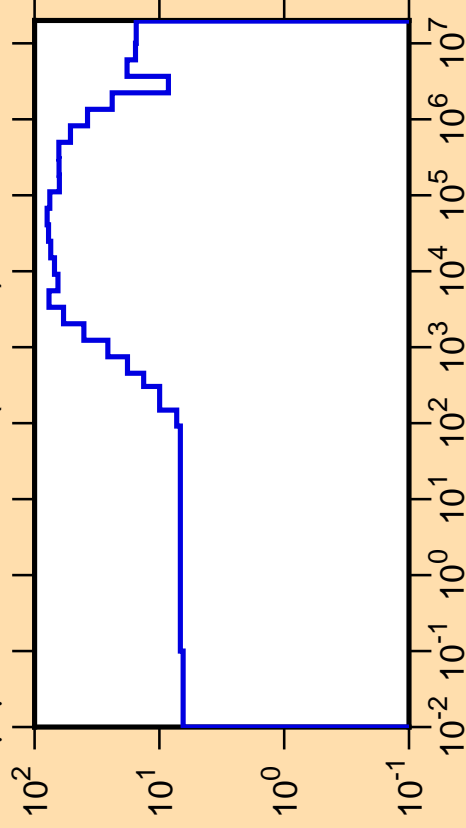
\Delta\mu/\mu vs. E for ^{122}\text{In}(\text{mt251})
