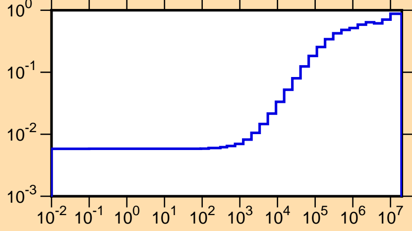
\mu vs. E for ^{122}\text{In}(\text{mt251})
