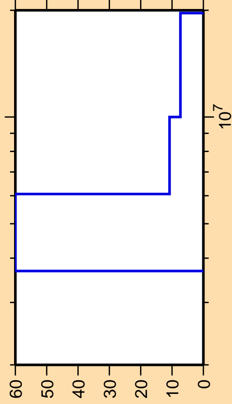
\Delta\sigma/\sigma vs. E for ^{122}\text{In}(n,2n)
