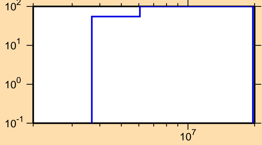
\Delta\sigma/\sigma vs. E for ^{122}\text{In}(n,n_1)
