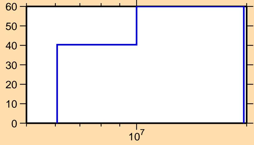
\Delta\sigma/\sigma vs. E for ^{122}\text{In}(n,ncont.)
