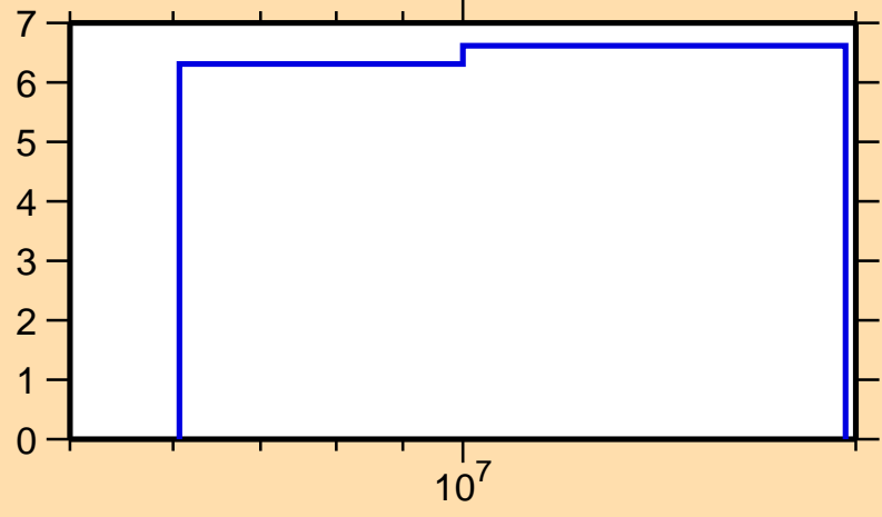
\Delta\sigma/\sigma vs. E for ^{122}\text{In}(n,\text{nonel.})
