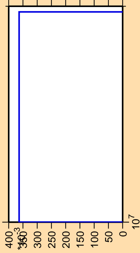
\Delta\sigma/\sigma vs. E for ^{122}\text{In}(n,2n\alpha)
