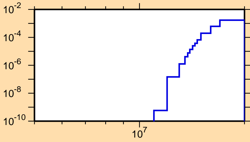
\sigma vs. E for ^{122}\text{In}(n,np)
