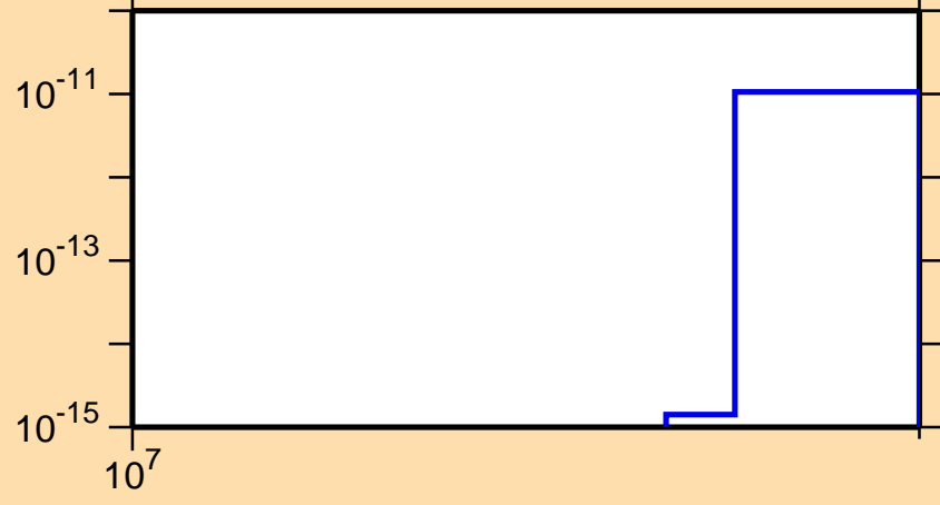
\sigma vs. E for ^{122}\text{In}(n,2n\alpha)
