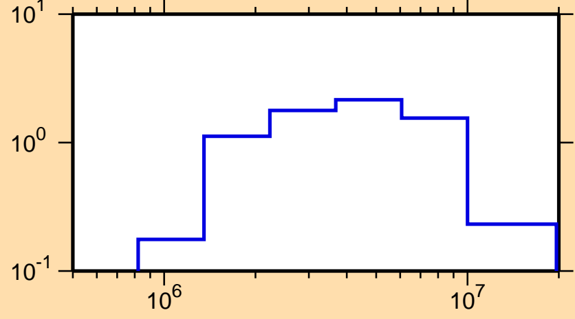
\sigma vs. E for ^{122}\text{In}(n,n\text{cont.})
