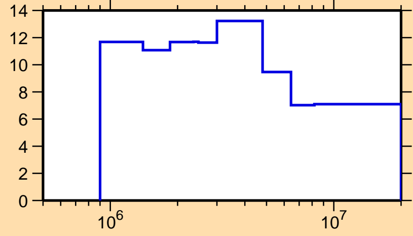
\Delta\sigma/\sigma vs. E for ^{122}\text{In}(n,n\text{nonel.})
