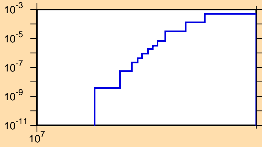
\sigma vs. E for ^{123}\text{In}(n,np)
