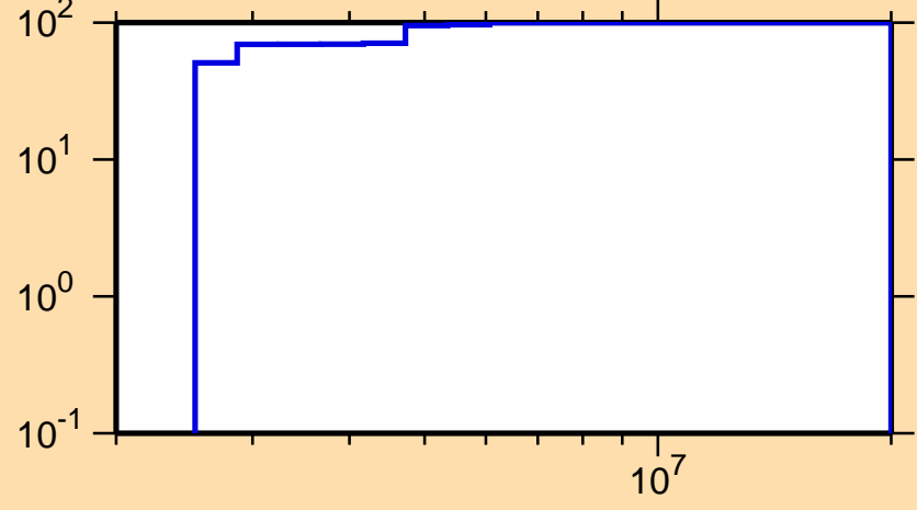
\Delta\sigma/\sigma vs. E for ^{123}\text{In}(n, n_1)
