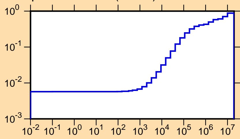
\mu vs. E for ^{123}\text{In}(\text{mt251})
