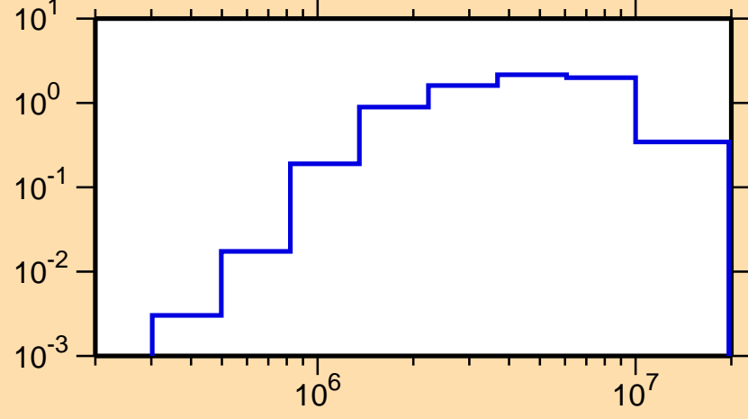
\sigma vs. E for ^{123}\text{In}(n,\text{inel.})
