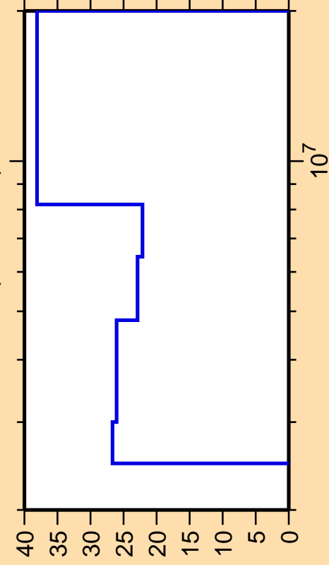
\Delta\sigma/\sigma vs. E for ^{123}\text{In}(n,n\text{cont.})
