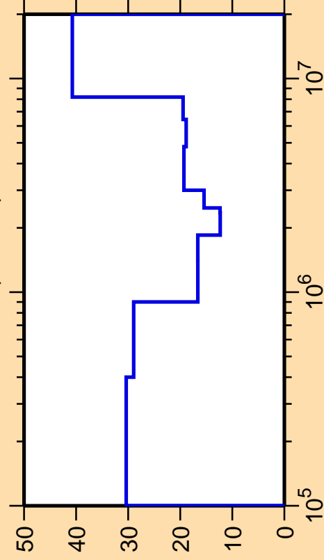
\Delta\sigma/\sigma vs. E for ^{123}\text{In}(n,\text{inel.})
