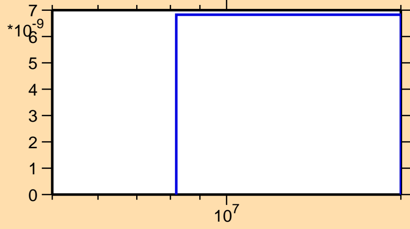
\sigma vs. E for ^{123}\text{In}(n,n\alpha)
