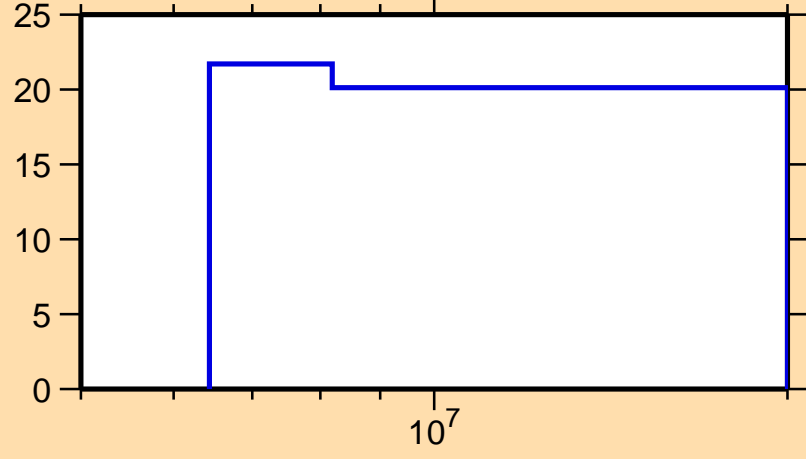
\Delta\sigma/\sigma vs. E for ^{123}\text{In}(n,\text{nonel.})
