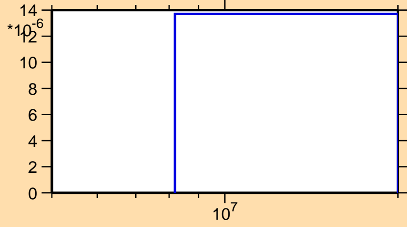
\sigma vs. E for ^{123}\text{In}(n,np)
