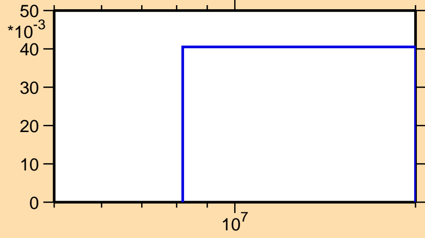
\sigma vs. E for ^{123}\text{In}(n,3n)
