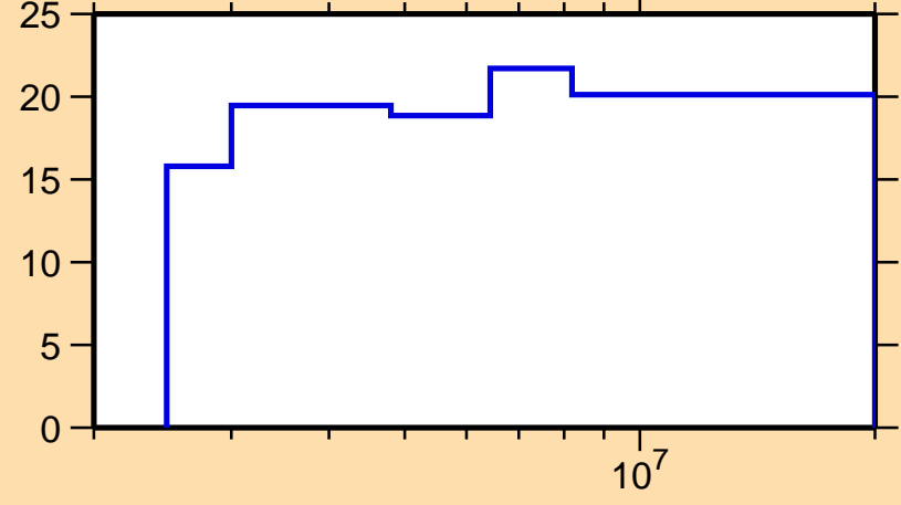
\Delta\sigma/\sigma vs. E for ^{123}\text{In}(n,n\text{nonel.})
