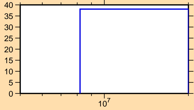
\Delta\sigma/\sigma vs. E for ^{123}\text{In}(n,n\text{cont.})
