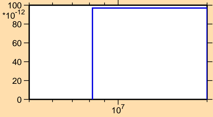
\sigma vs. E for ^{123}\text{In}(n,nt)
