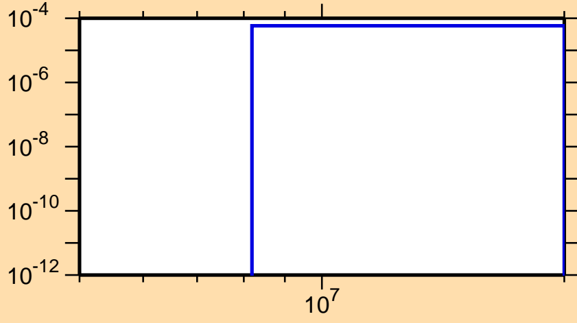
\sigma vs. E for ^{123}\text{In}(n,d)
