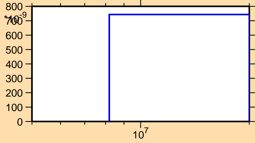
\sigma vs. E for ^{123}\text{In}(n,t)
