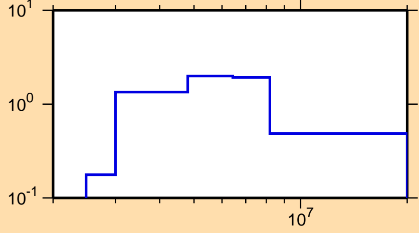
\sigma vs. E for ^{123}\text{In}(n,n\text{cont.})
