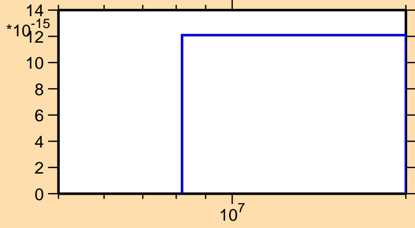
\sigma vs. E for ^{123}\text{In}(n,2np)
