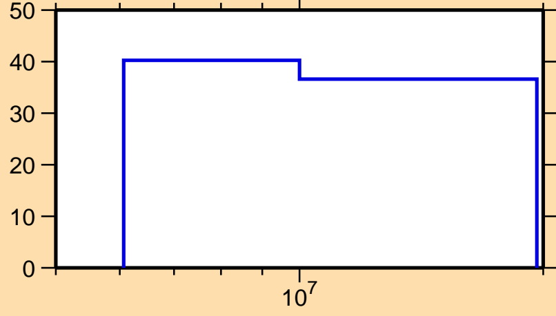
\Delta\sigma/\sigma vs. E for ^{123}\text{In}(n,el.)
