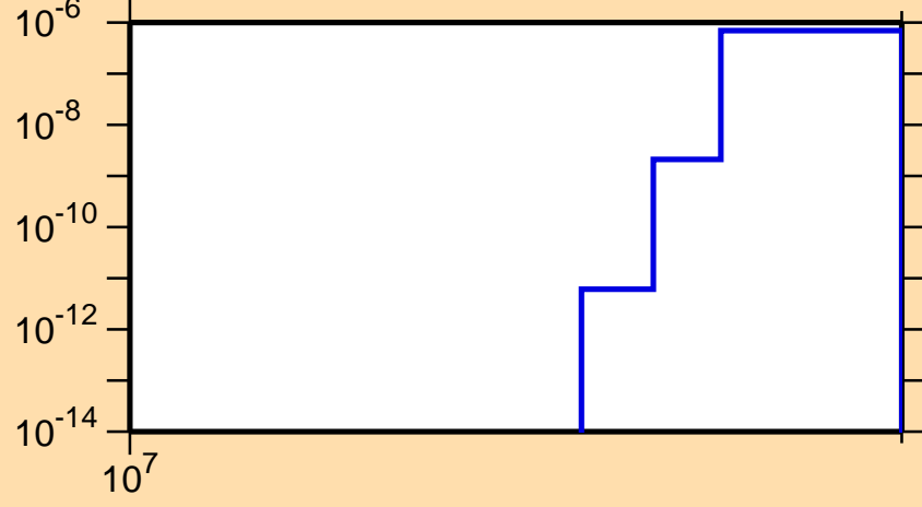
\sigma vs. E for ^{124}\text{In}(n,\text{nd})
