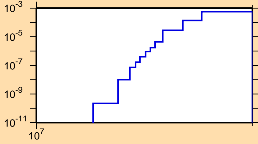
\sigma vs. E for ^{124}\text{In}(n,np)
