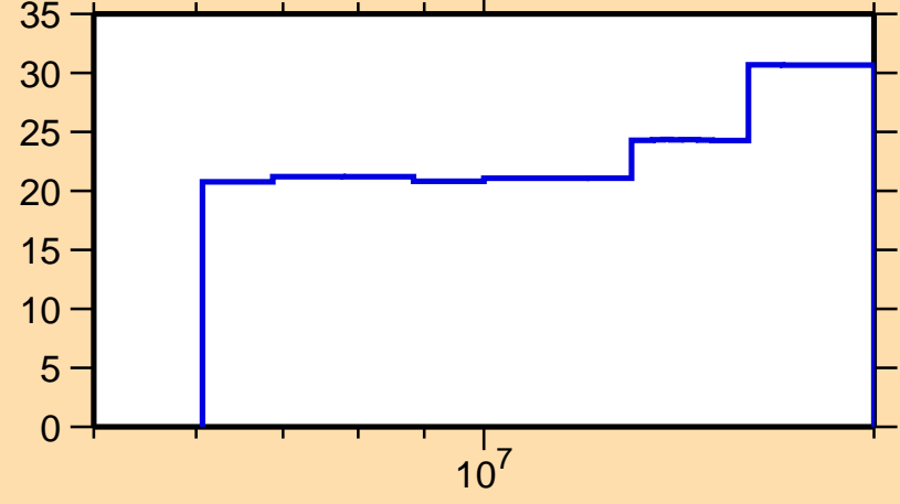
\Delta\sigma/\sigma vs. E for ^{124}\text{In}(n,\text{nonel.})
