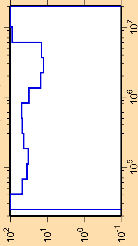
\Delta\sigma/\sigma vs. E for ^{124}\text{In}(n,\text{inel.})
