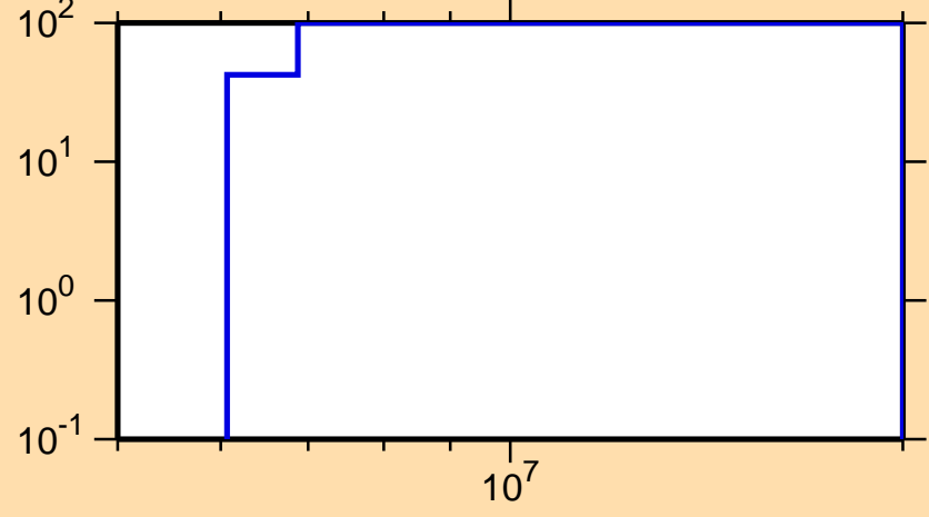
\Delta\sigma/\sigma vs. E for ^{124}\text{In}(n,n\text{cont.})
