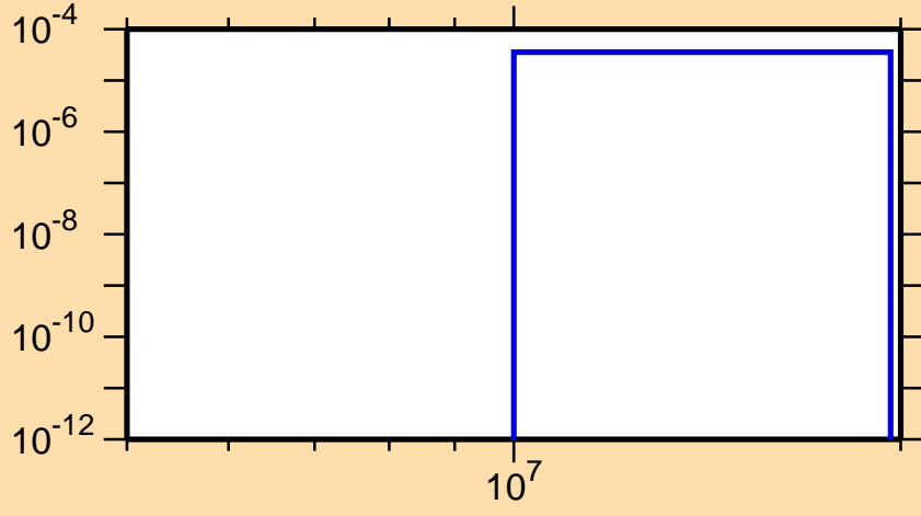
\sigma vs. E for ^{124}\text{In}(n,d)
