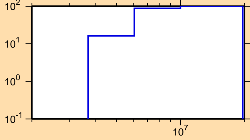
\Delta\sigma/\sigma vs. E for ^{124}\text{In}(n,ncont.)
