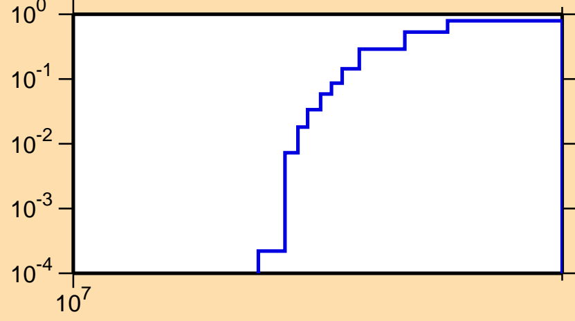
\sigma vs. E for ^{125}\text{In}(n,3n)
