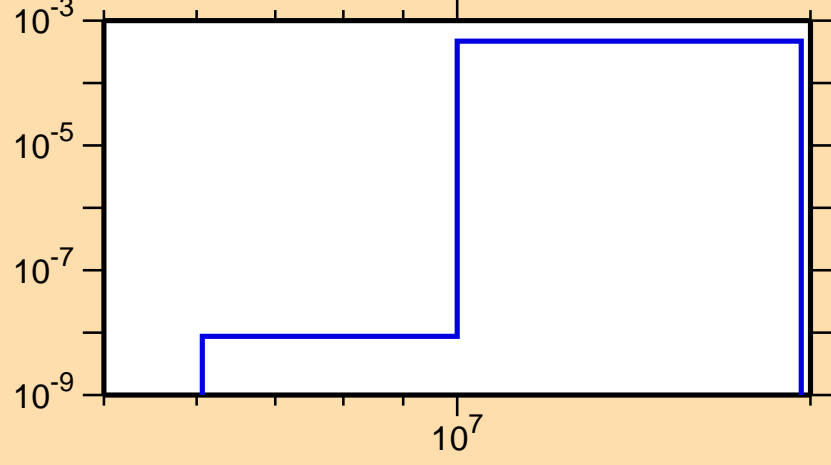
\sigma vs. E for ^{125}\text{In}(n,p)
