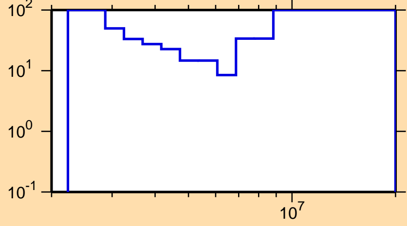
\Delta\sigma/\sigma vs. E for ^{125}\text{In}(n,n\text{cont.})
