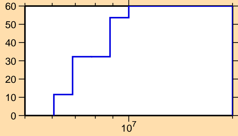
\Delta\sigma/\sigma vs. E for ^{126}\text{In}(n,ncont.)
