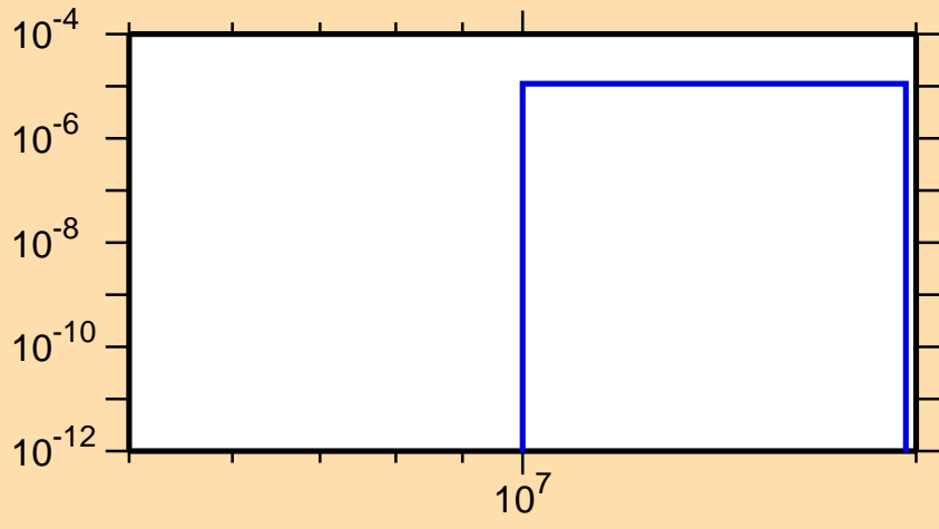
\sigma vs. E for ^{126}\text{In}(n,d)
