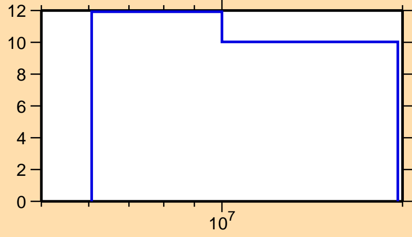
\Delta\sigma/\sigma vs. E for ^{126}\text{In}(n,el.)
