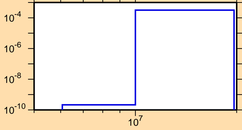
\sigma vs. E for ^{126}\text{In}(n,p)
