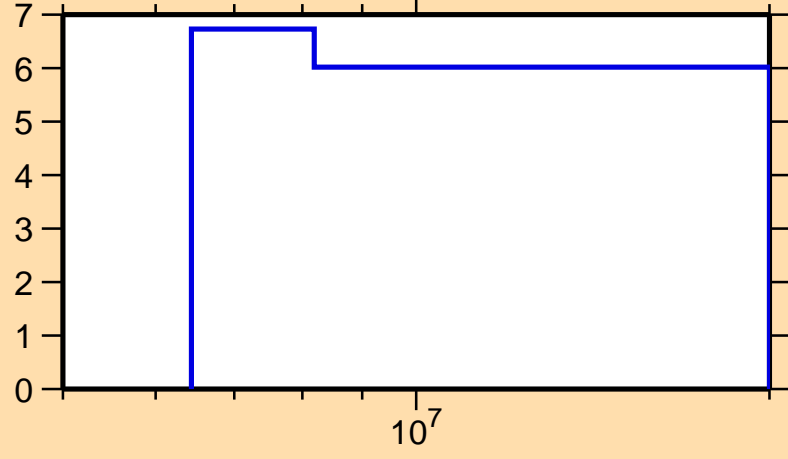
\Delta\sigma/\sigma vs. E for ^{126}\text{In}(n,\text{tot.})
