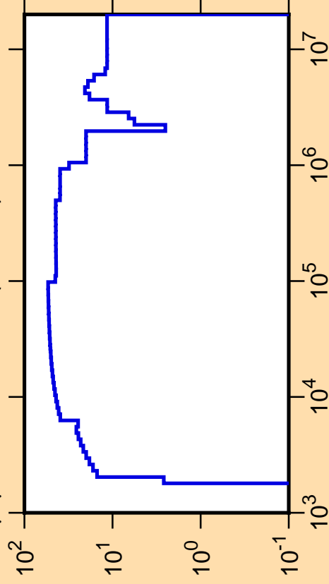
\Delta\mu/\mu vs. E for ^{127}\text{In}(\text{mt251})
