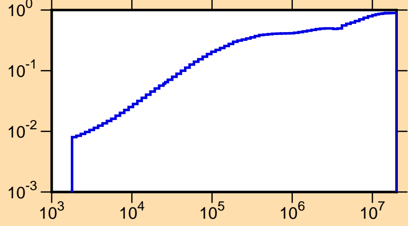
\mu vs. E for ^{127}\text{In}(\text{mt251})
