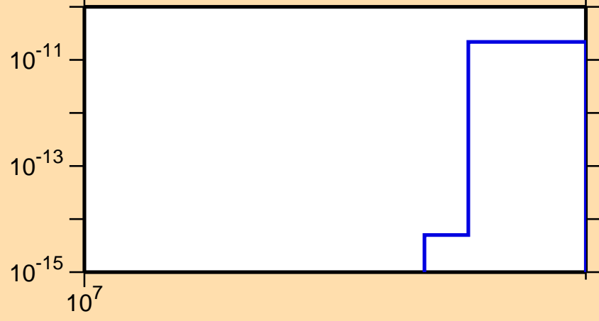
\sigma vs. E for ^{127}\text{In}(n,\text{nd})
