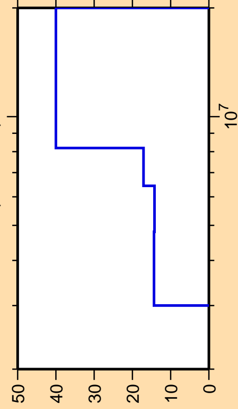
\Delta\sigma/\sigma vs. E for ^{127}\text{In}(n,\text{ncont.})
