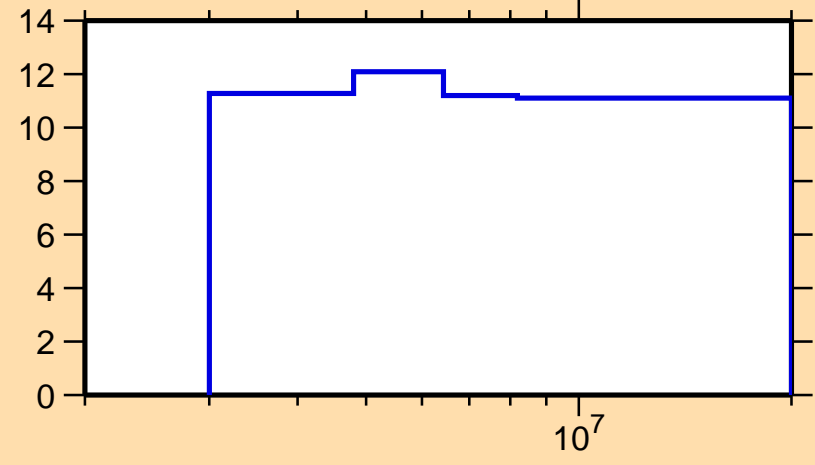
\Delta\sigma/\sigma vs. E for ^{127}\text{In}(n,n\text{nonel.})
