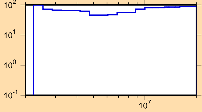
\Delta\sigma/\sigma vs. E for ^{127}\text{In}(n,n\text{cont.})
