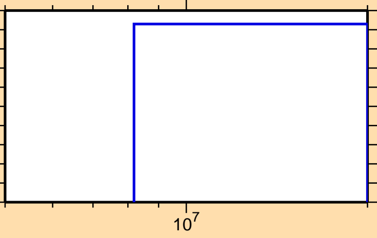
\sigma vs. E for ^{127}\text{In}(n,np)
