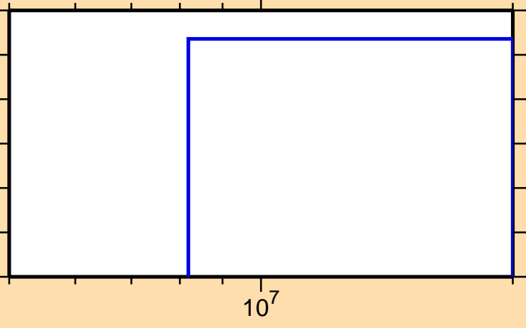
\sigma vs. E for ^{127}\text{In}(n,3n)
