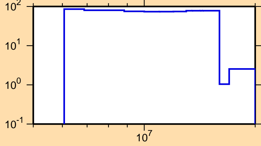
\Delta\sigma/\sigma vs. E for ^{127}\text{In}(n,n_1)
