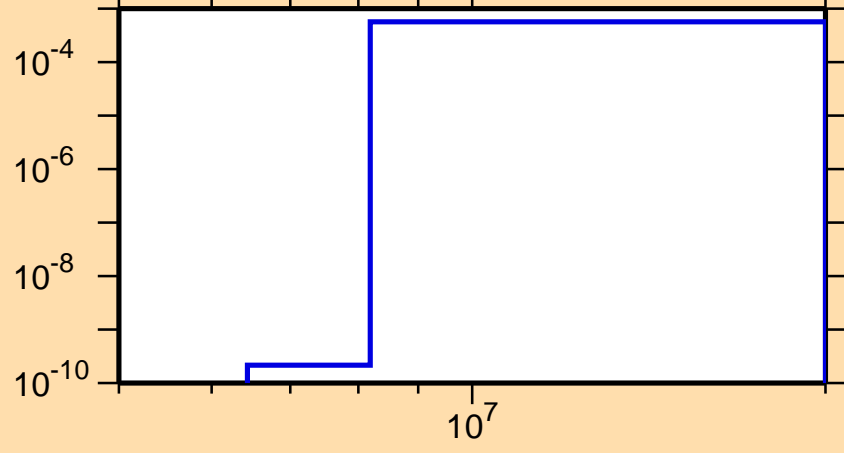
\sigma vs. E for ^{127}\text{In}(n,p)
