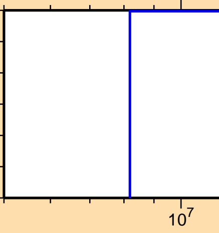
\sigma vs. E for ^{127}\text{In}(\text{mt } 11)
