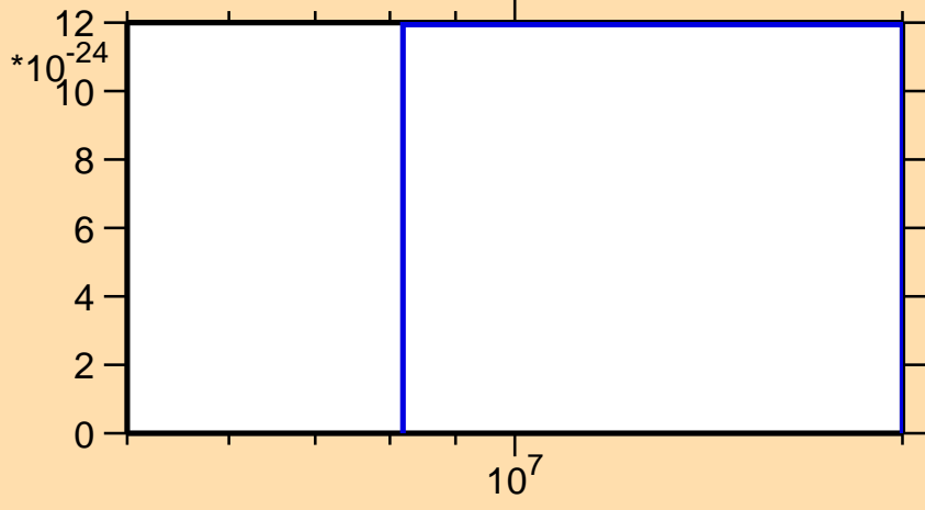
\sigma vs. E for ^{127}\text{In}(\text{mt } 11)
