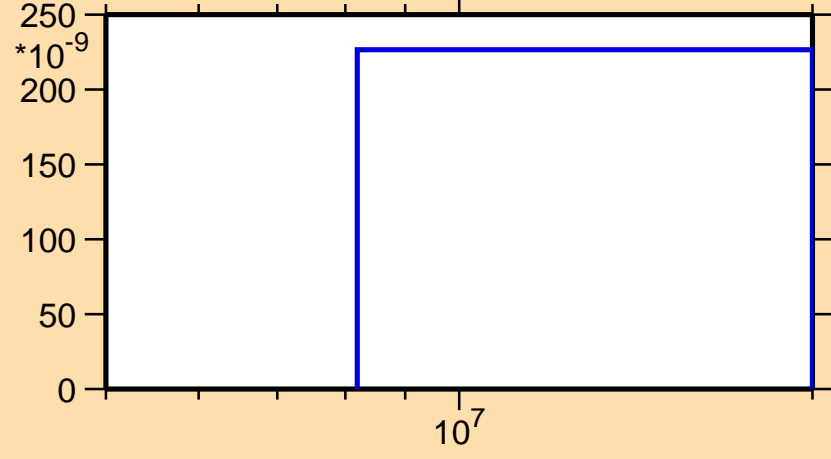
\sigma vs. E for ^{129}\text{In}(n,d)
