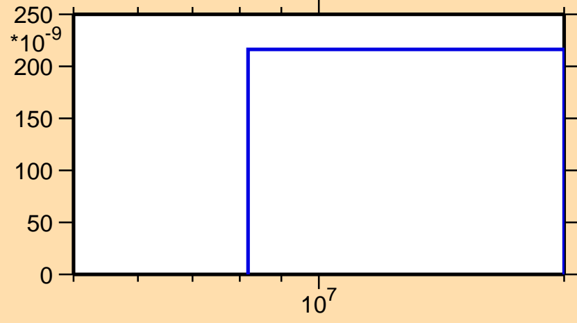
\sigma vs. E for ^{129}\text{In}(n,np)
