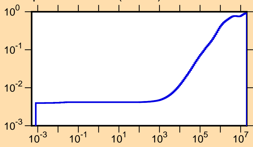
\mu vs. E for ^{171}\text{Ir}(\text{mt251})
