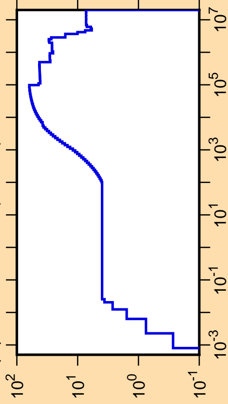
\Delta\mu/\mu vs. E for ^{171}\text{Ir}(\text{mt251})
