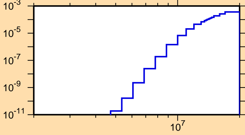
\sigma vs. E for ^{171}\text{Ir}(\text{mt117})
