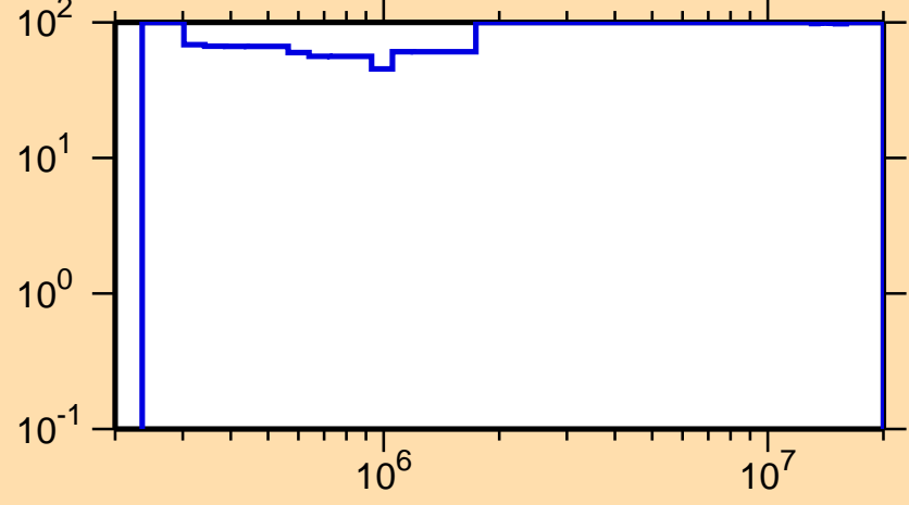
\Delta\sigma/\sigma vs. E for ^{171}\text{Ir}(n,n_1)
