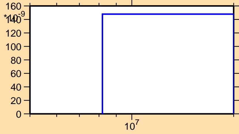
\sigma vs. E for ^{171}\text{Ir}(n,\text{nd})
