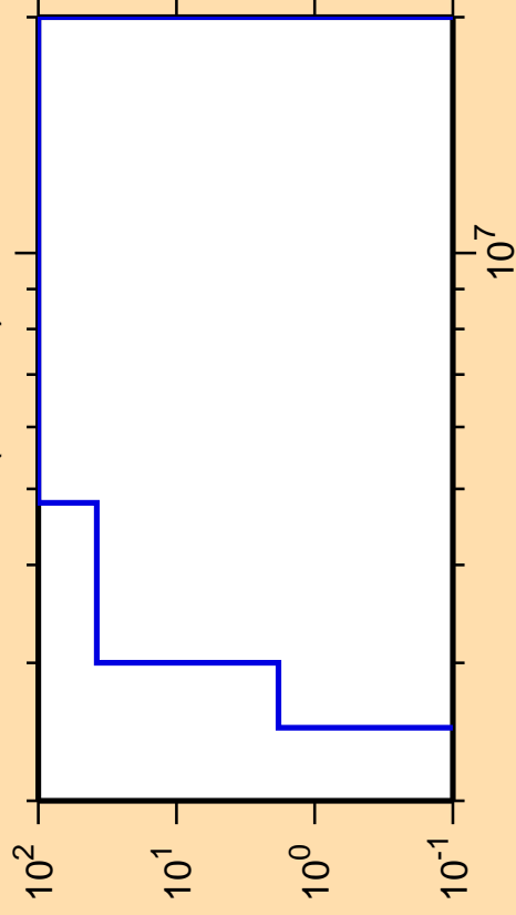
\Delta\sigma/\sigma vs. E for ^{171}\text{Ir}(n,\text{He}3)
