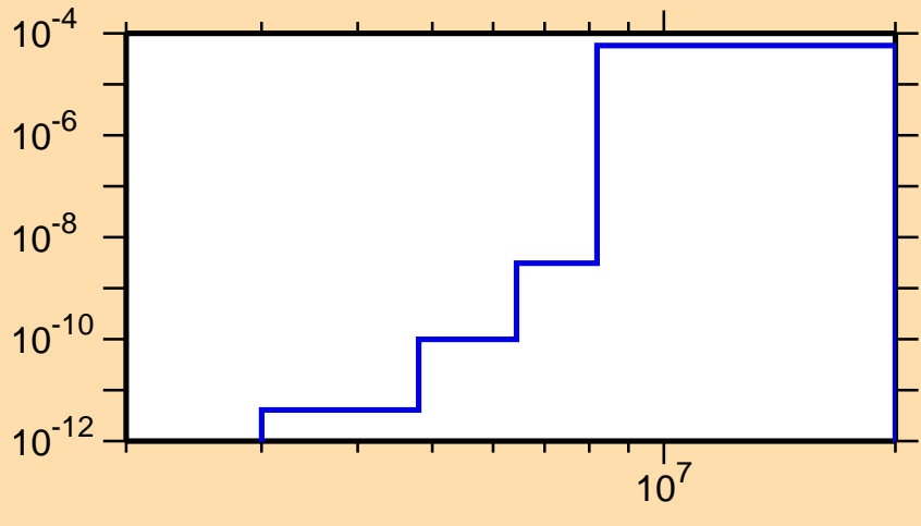
\sigma vs. E for ^{171}\text{Ir}(n,\text{He}3)
