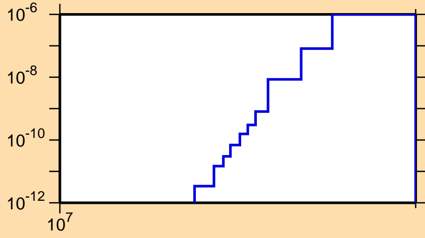
\sigma vs. E for ^{171}\text{Ir}(n,\text{pt})
