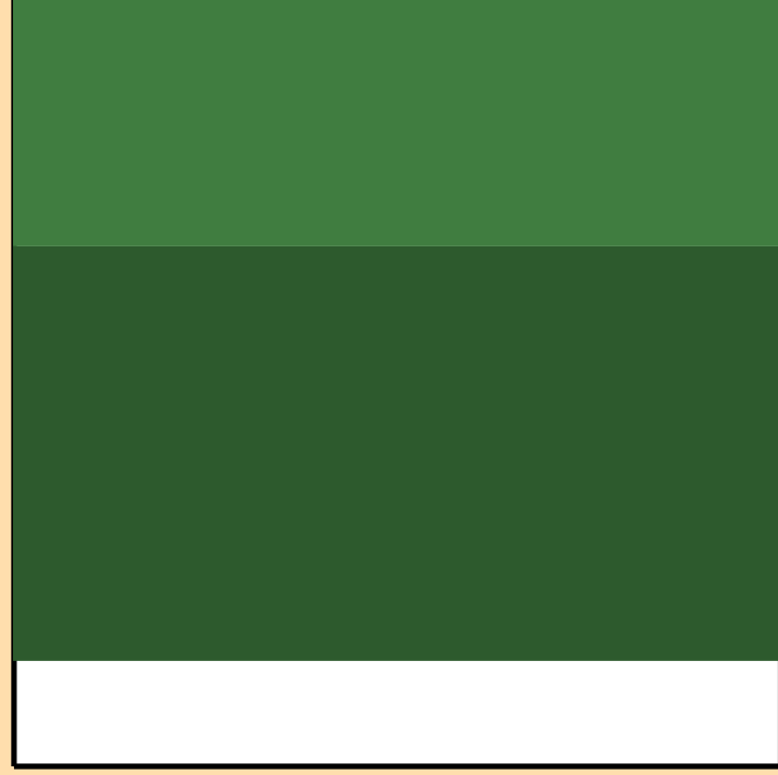
\Delta\sigma/\sigma vs. E for ^{171}\text{Ir}(n,\text{nonel.})
