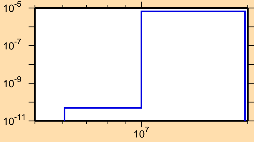
\sigma vs. E for ^{171}\text{Ir}(n,\text{pd})
