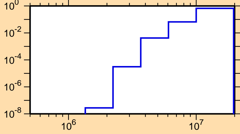
\sigma vs. E for ^{171}\text{Ir}(n,np)
