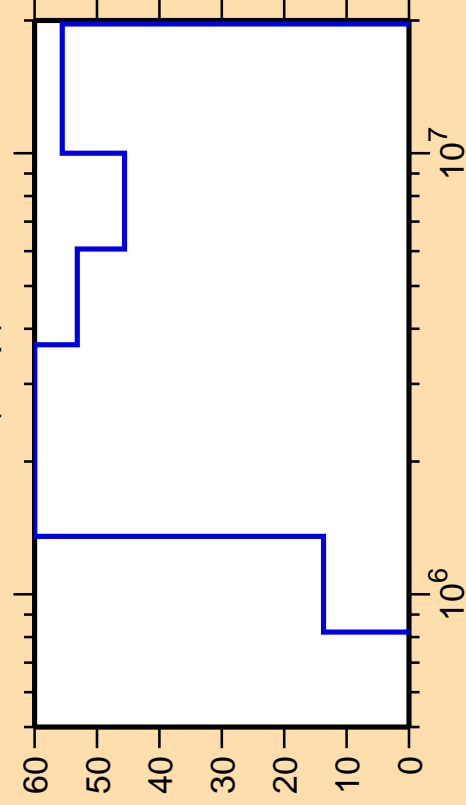
\Delta\sigma/\sigma vs. E for ^{171}\text{Ir}(n,np)
