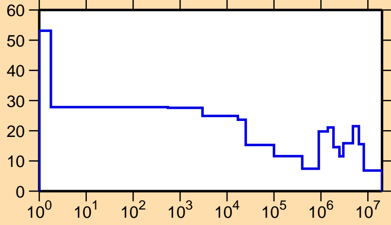
\Delta\sigma/\sigma vs. E for ^{171}\text{Ir}(n,\text{el.})
