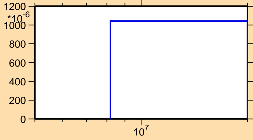
\sigma vs. E for ^{171}\text{Ir}(n,2n\alpha)
