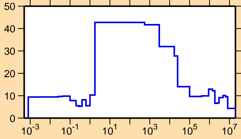
\Delta\sigma/\sigma vs. E for ^{171}\text{Ir}(n,\text{tot.})
