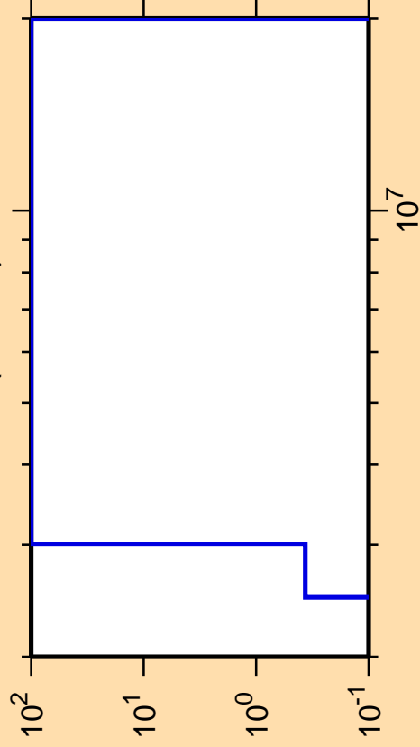
\Delta\sigma/\sigma vs. E for ^{171}\text{Ir}(\text{mt117})
