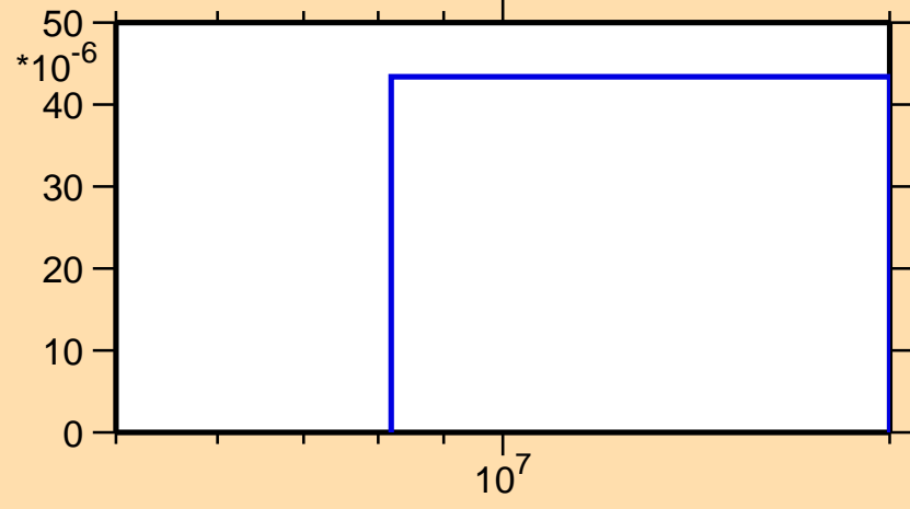
\sigma vs. E for ^{171}\text{Ir}(n,2np)
