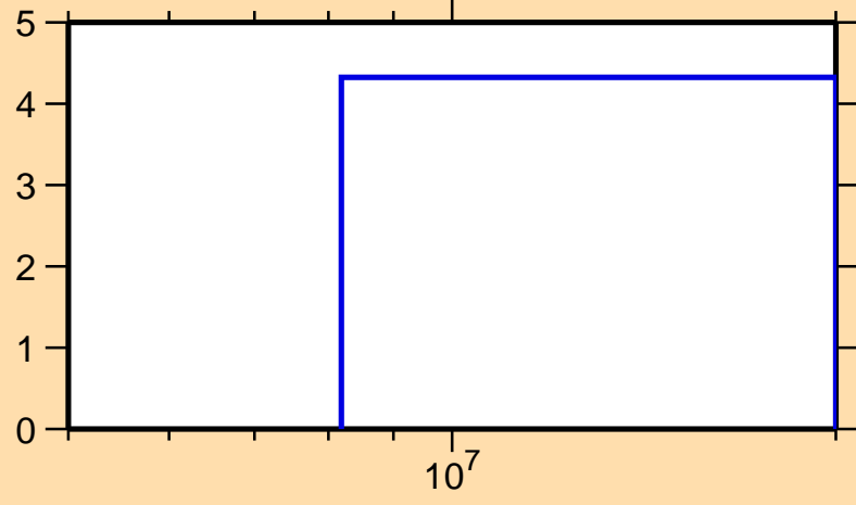
\Delta\sigma/\sigma vs. E for ^{171}\text{Ir}(n,\text{tot.})
