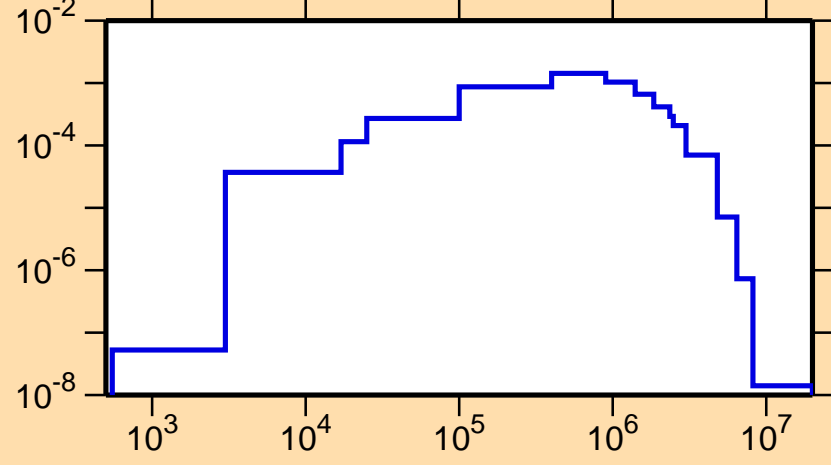
\sigma vs. E for ^{171}\text{Ir}(n,n_2)
