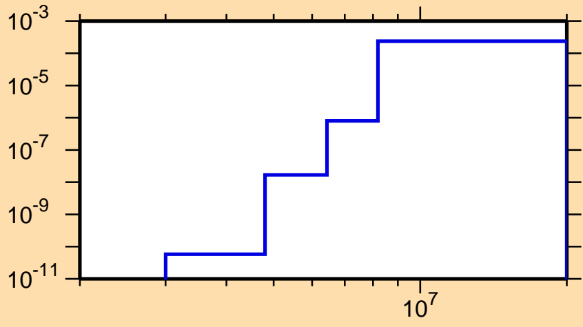
\sigma vs. E for ^{171}\text{Ir}(\text{mt117})
