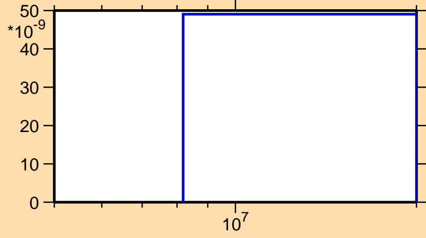
\sigma vs. E for ^{171}\text{Ir}(n,\text{nd})
