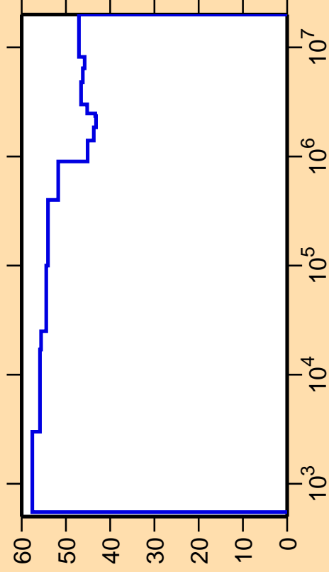
\Delta\sigma/\sigma vs. E for ^{171}\text{Ir}(n,n_2)
