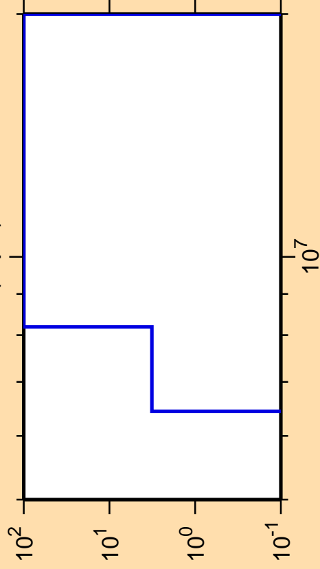
\Delta\sigma/\sigma vs. E for ^{171}\text{Ir}(n,\text{pd})
