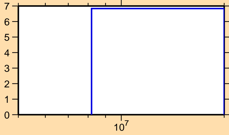
\Delta\sigma/\sigma vs. E for ^{171}\text{Ir}(n,\text{el.})
