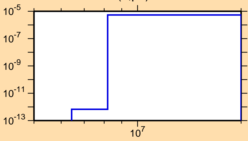
\sigma vs. E for ^{171}\text{Ir}(n,\text{pd})
