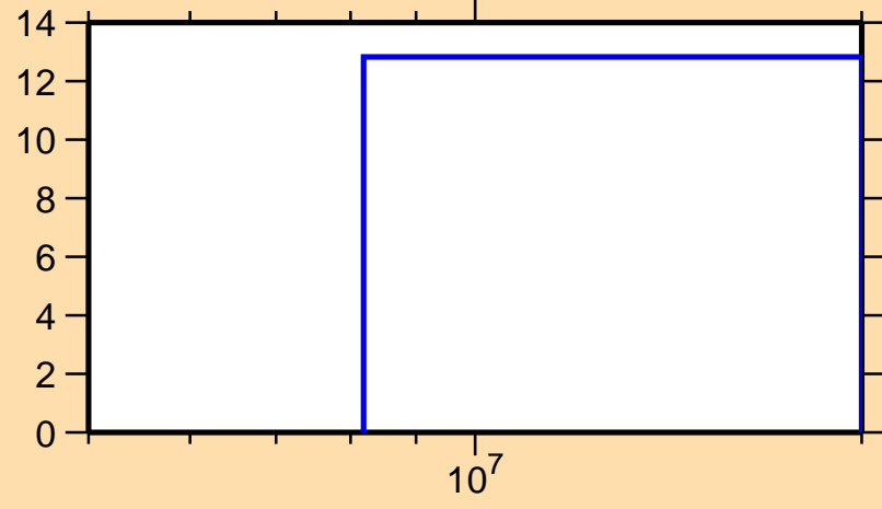
\Delta\sigma/\sigma vs. E for ^{171}\text{Ir}(n,\text{nonel.})
