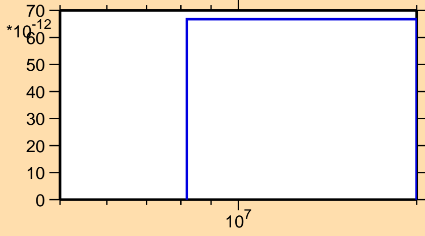
\sigma vs. E for ^{171}\text{Ir}(n,nt)
