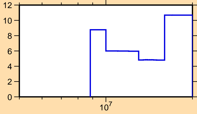
\Delta\sigma/\sigma vs. E for ^{172}\text{Ir}(n,\text{el.})
