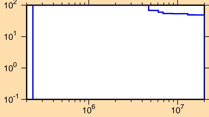
\Delta\sigma/\sigma vs. E for ^{172}\text{Ir}(n,n\text{cont.})
