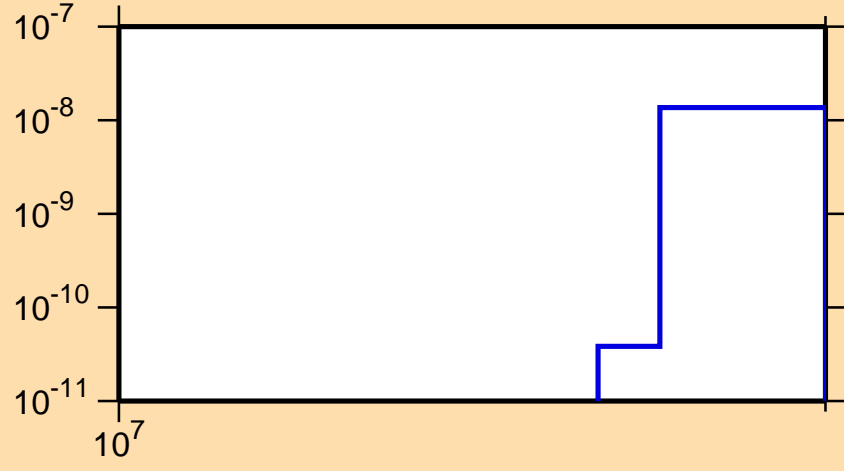
\sigma vs. E for ^{172}\text{Ir}(n,nt)
