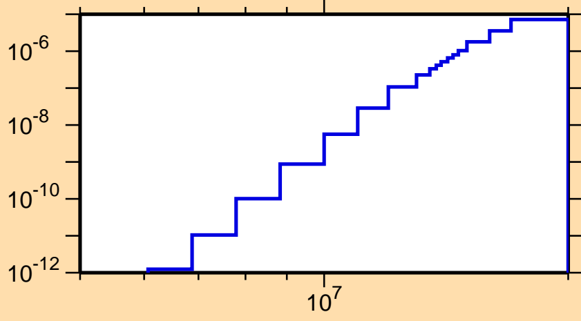
\sigma vs. E for ^{172}\text{Ir}(\text{mt117})
