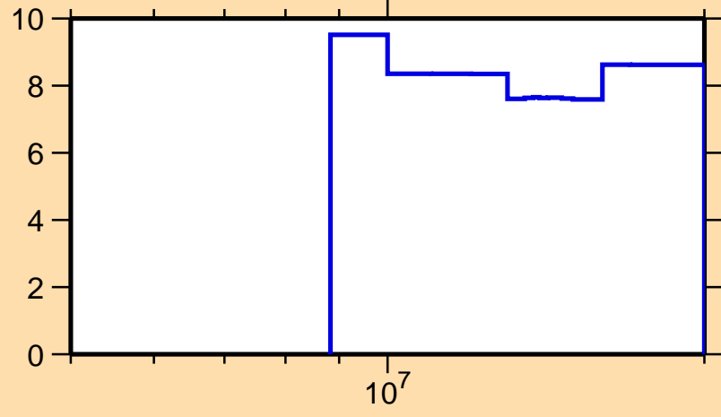
\Delta\sigma/\sigma vs. E for ^{172}\text{Ir}(n,\text{tot.})
