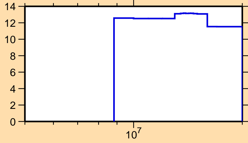
\Delta\sigma/\sigma vs. E for ^{172}\text{Ir}(n,\text{nonel.})
